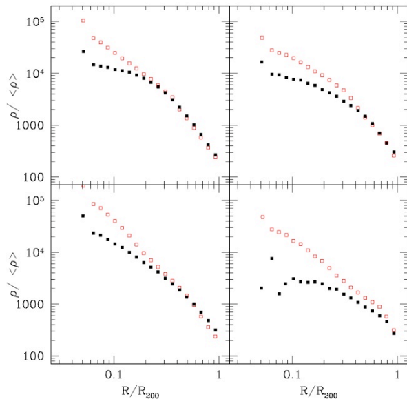
Gas density profiles for preheat (black) and nocool (red), for matched halos.
