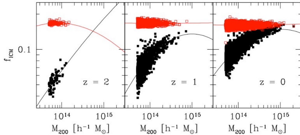
f_{\text{ICM}} for preheat (black) and nocool (red)
