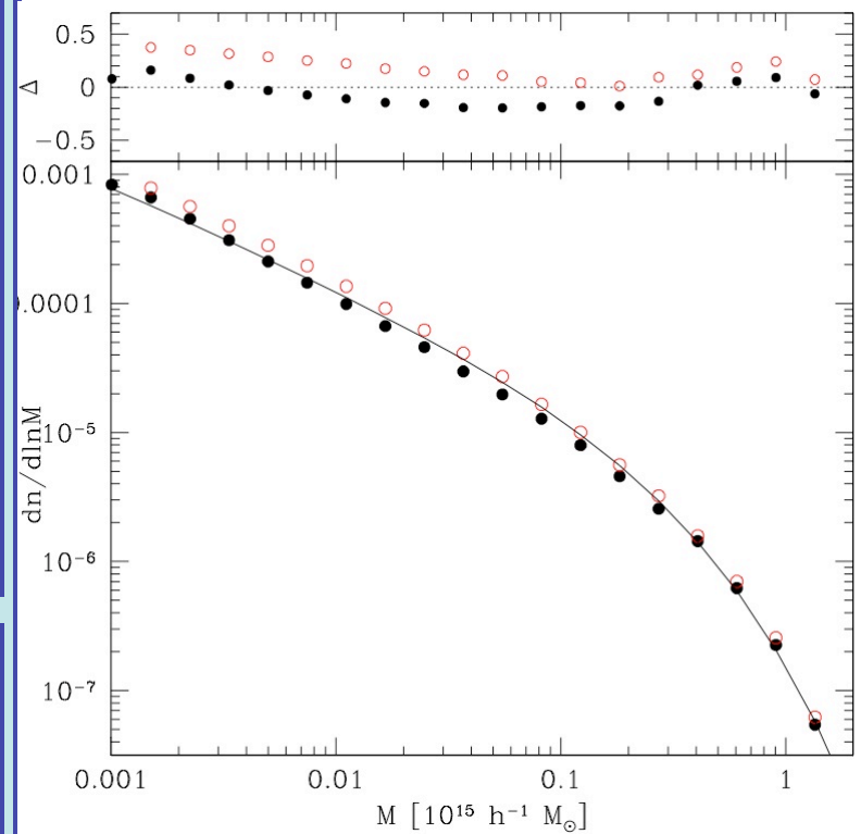
Halo total mass function for preheat (black) and nocool (red) at z = 0 . Note the 20% difference at low mass.
